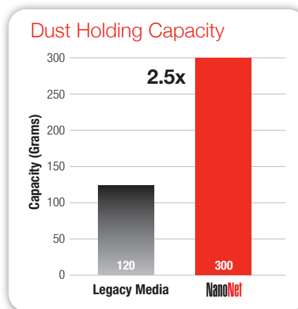
Primary fuel filter for mid-range diesel engine.
